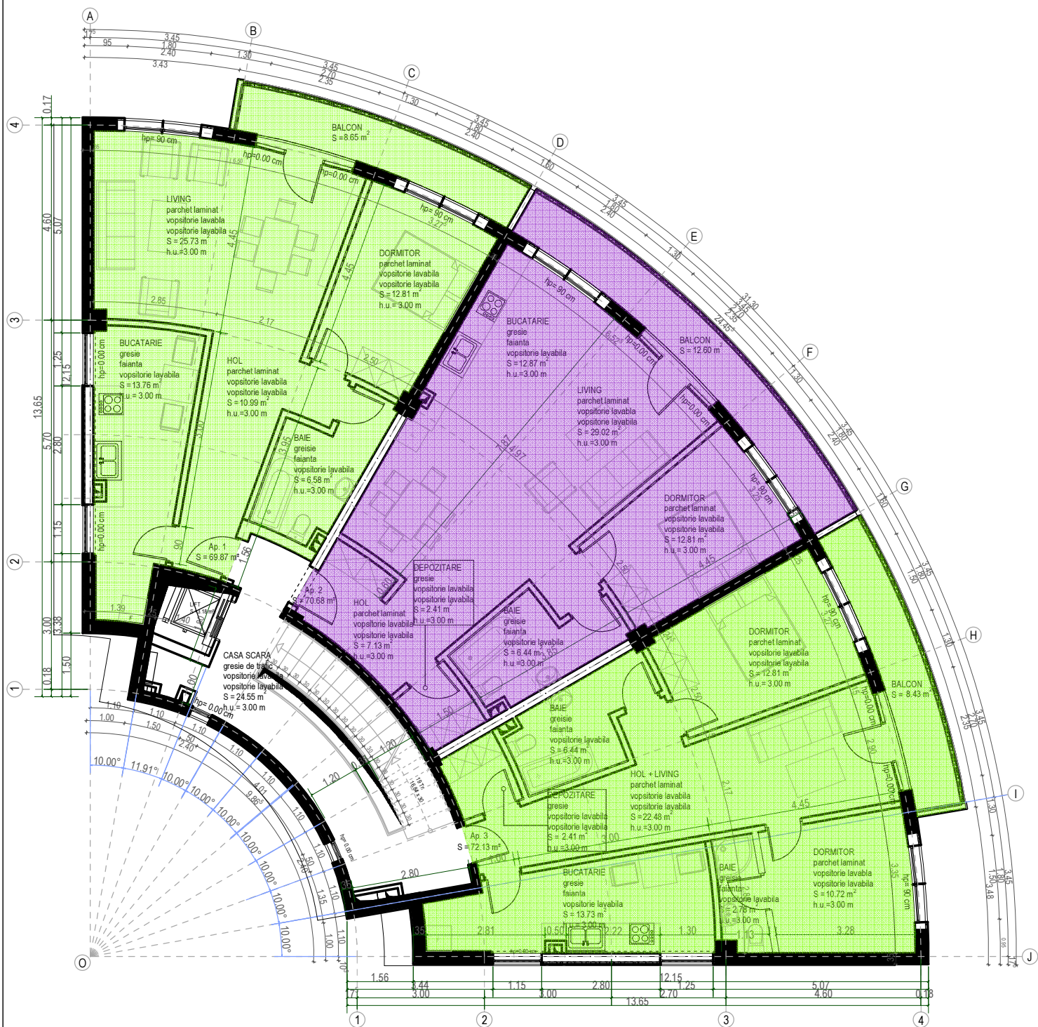
PLAN ETAJ CURENT 1-6 S = 278.66 m 2
